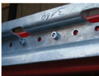
Figur 11: Ankerskinne
